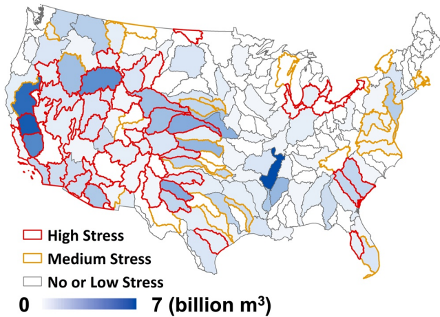
Figure 4. Total blue water footprint of Food-Energy-Water (FEW) production for watersheds across the United States with corresponding water stress levels. Here, watersheds are defined following the 4-digit Hydrologic Unit Code. Water stress is shown by the watershed boundary colors, while the blue fill shows the total blue water footprint of FEW production within the watershed.
